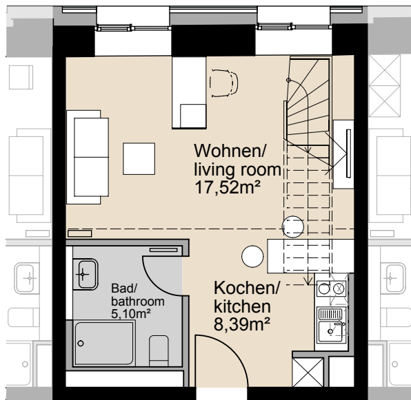
3. Obergeschoss/ 3rd floor
